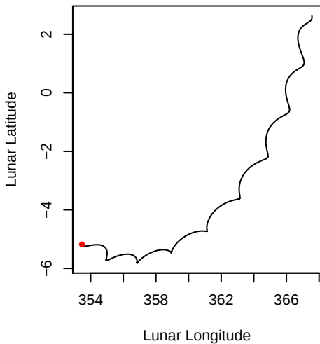
Sub-radar point
