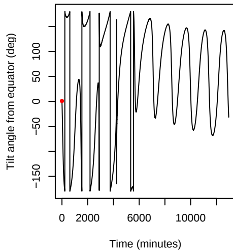
Doppler Equator
