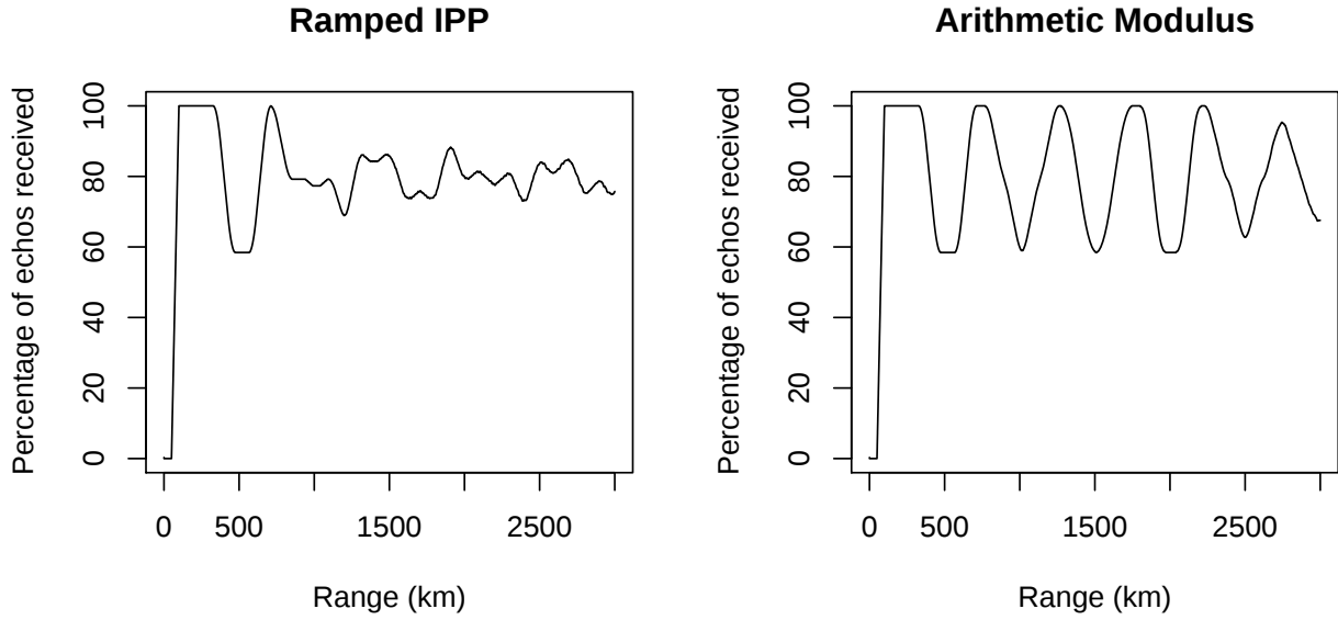
Figure 1. A comparison of ramped IPP ( N = 53 , a = 84 \times 30 , k = 30 ), and arithmetic modulus coding ( p = 1590 , a = 84 \times 30 , k = 14 \times 30 ) radar efficiency per range. Both experiments have the same duty-cycle and transmission length. The ramped IPPs show less variation in radar efficiency than the arithmetic modulus coding above 1000 km.
