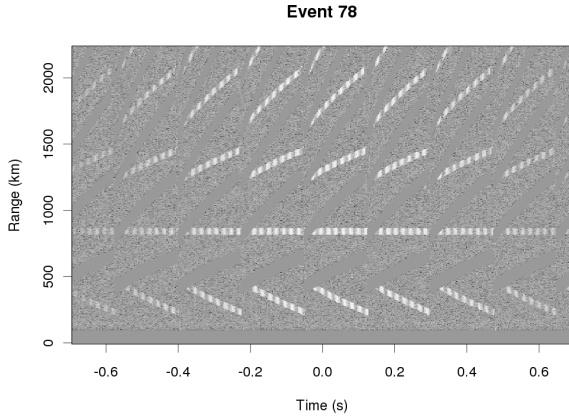
Figure 2. The raw zero-lag echoes from a single event at around 800 km. The gray uniformly colored regions are transmission slots from which we do not get echoes. However, due to the non-uniform nature of the IPPs, we get some echoes from each range during one 0.17 s IPP cycle. The ambiguous echoes are ones that fan out around the correct echo. The backscatter cross-section is also fluctuating in a regular manner, most likely caused by an irregularly shaped object that is rotating.
